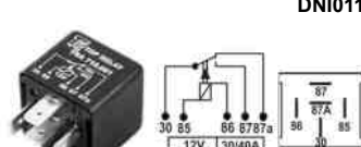
RELE AUX 12V 5T 30/40A - S/S TRA710081
