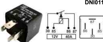
RELE AUX 12V 4T 40A S/S UNIVERSAL TRA111201
