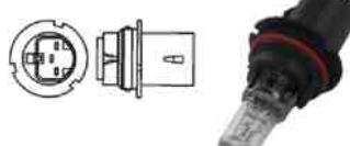
THB5 HB5 45/65W (9007)
