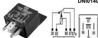
RELE AUX 12V 5T 10/40A C/S TRME700012
