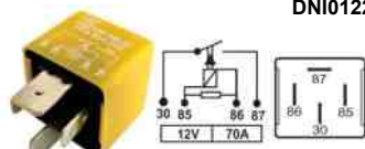
RELE AUX 12V 4T 70A C/S 2 LARGOS 2 FINOS TRA712170
