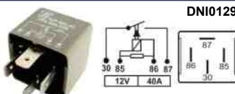
RELE BOMBA VW GM FORD HYD KIA LIFAN 4T TRA900000
