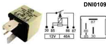
RELE BOMBA VW SANTANA GOLF AUDI 4T TRA108109
