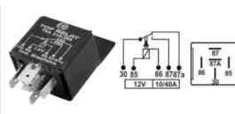
RELE AUX 12V 5 TERM 10/40A C/ SUPORTE TRA116203
