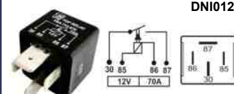
RELE AUX 12V 4T 70A S/S 2 LARGOS E 2 FINOS TRA712070
