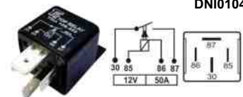
RELE AUX 12V 4T 50A C/S 2 LARGOS 2 FINOS TRA108400
